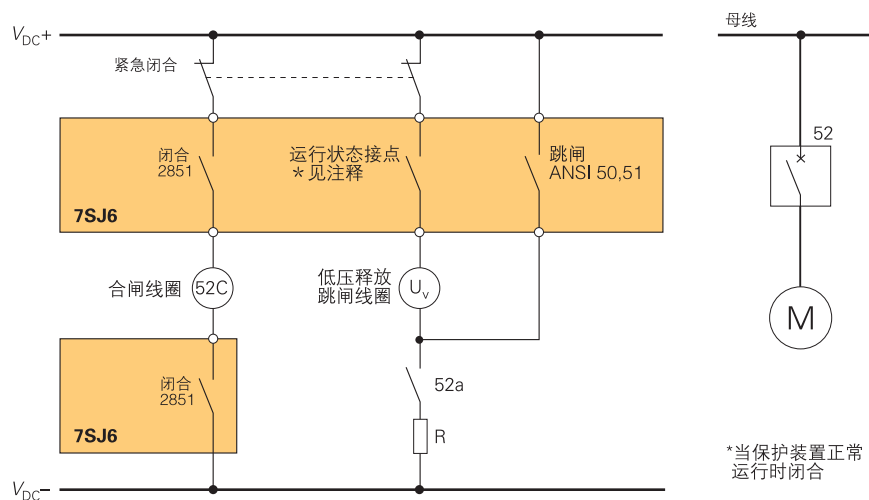
图5/133: 带50, 51接点的欠压释放
